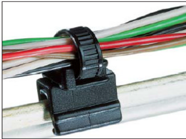
T50ROSEC4A - the cable bundle runs parallel with the edge.
