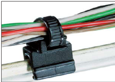
T50ROSEC4A - the cable bundle runs parallel with the edge.
