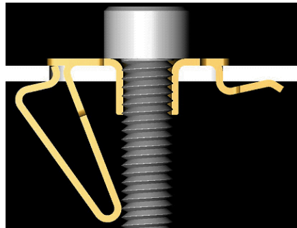
During installation of the bolt, the adjacent snap in feature is able to deflect and provide additional panel clamping.
